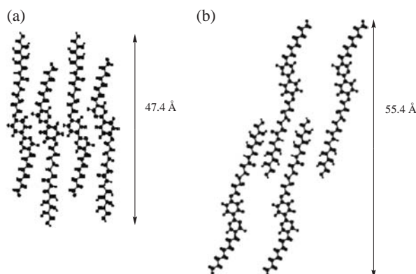
Figure 3. Molecular organization model for the SmA phase (a) and for the SmX phase (b).
