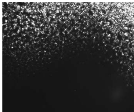
Figure 2. Photomicrograph of the SmA to SmX phase transition of a homeotropically aligned sample of compound 1 .
